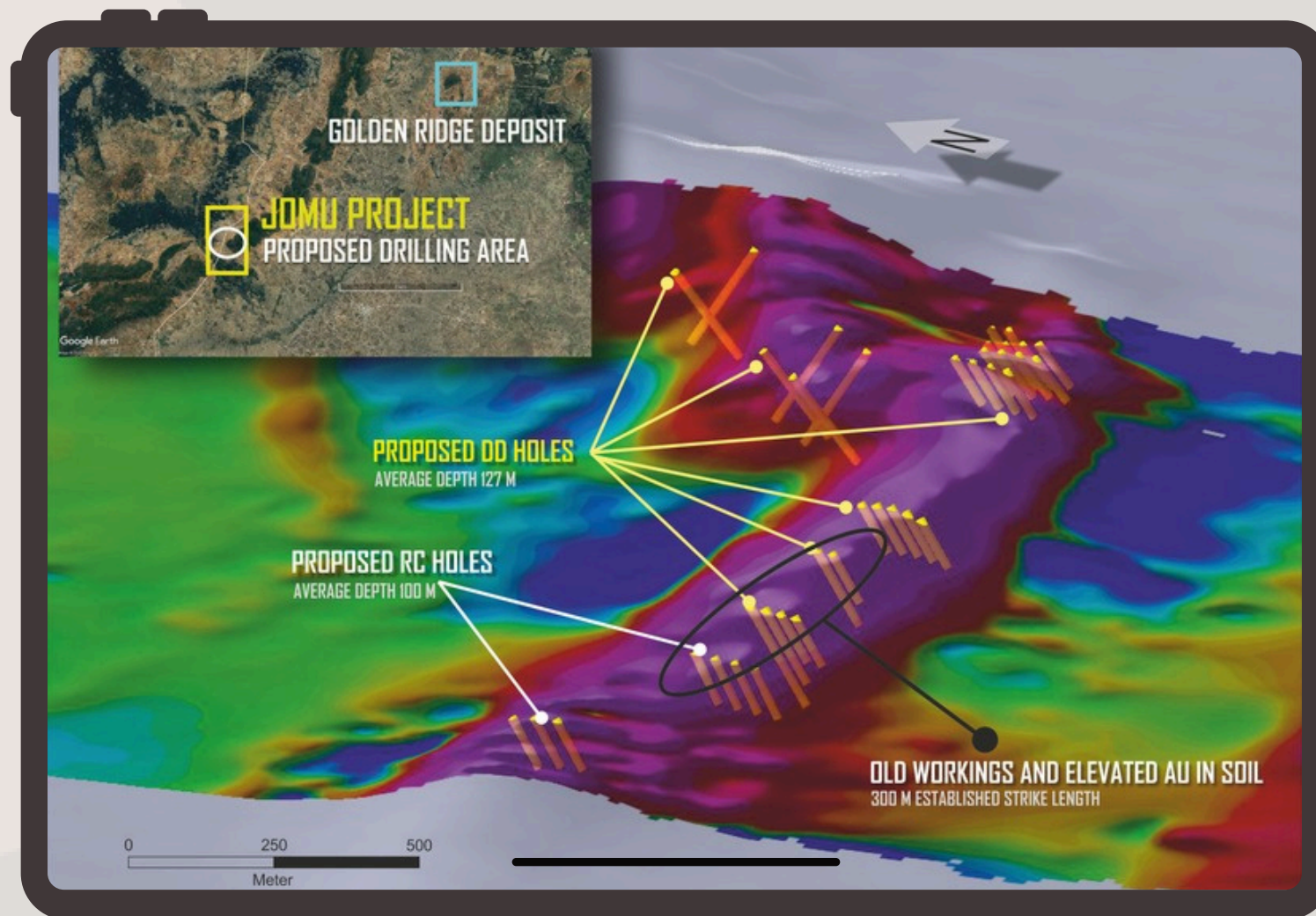
3D view of Borehole location map
