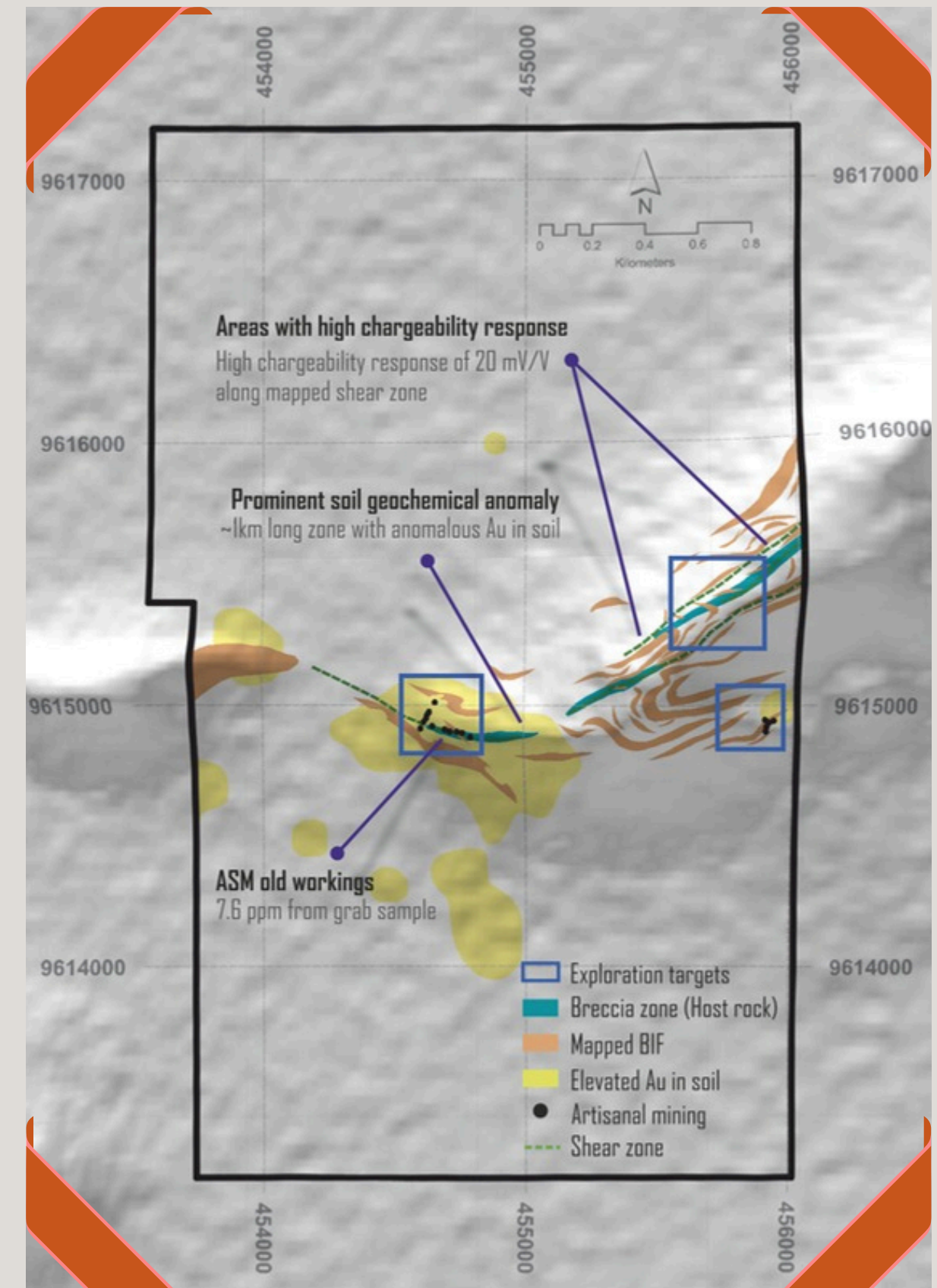
Geological Map of Jomu Gold Project
