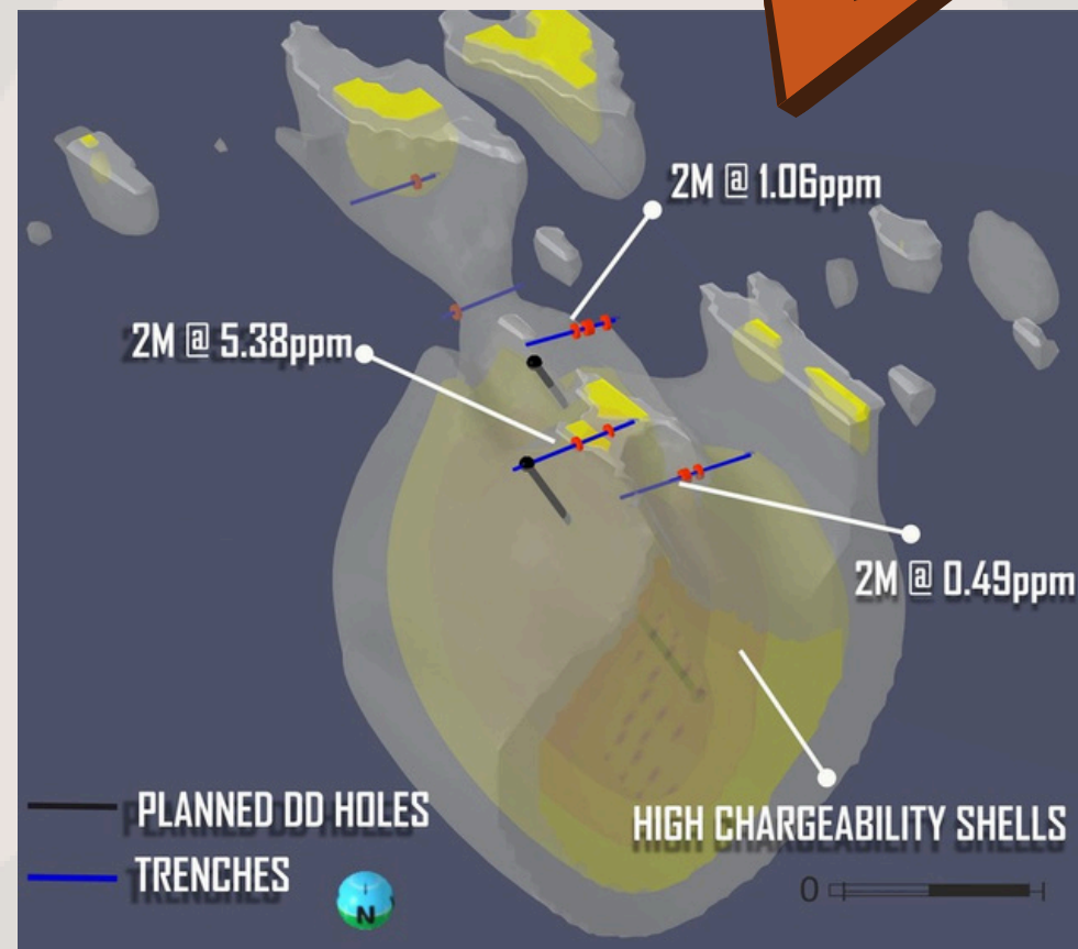
3D view of IPR surveyed results for one block
